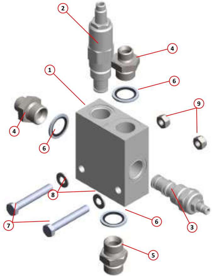
POWER STEERING REGULATOR VALVE (HYDRAFORCE)
