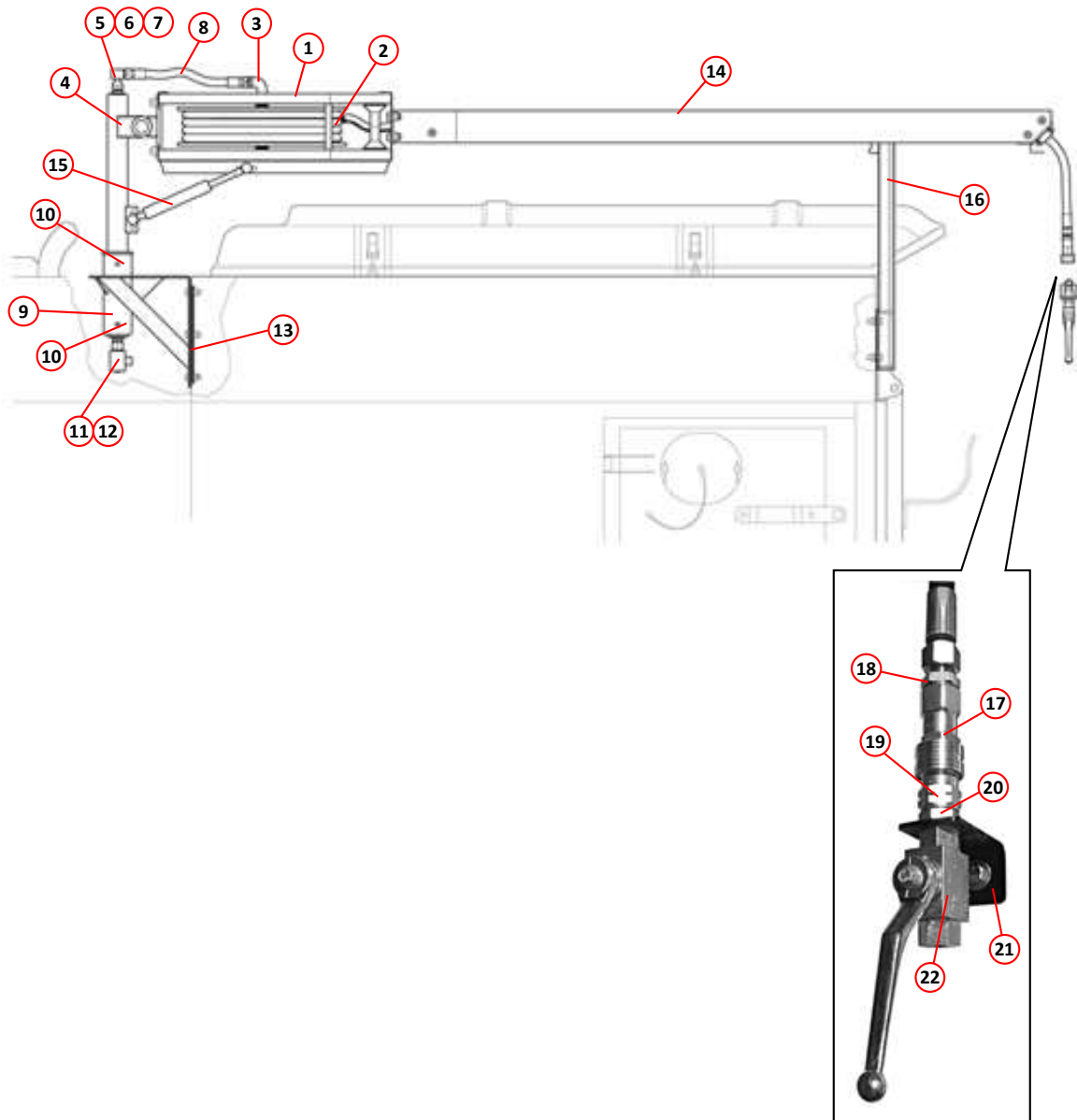
HIGH PRESSURE WATER BOOM ARRANGEMENT
