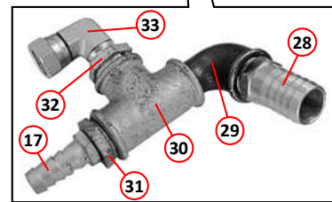
HIGH PRESSURE WATER PUMP - ARRANGEMENT
