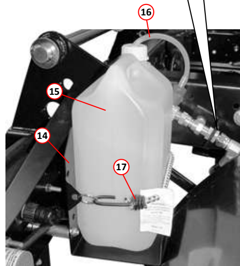
DETERGENT BOTTLE AND FEED VALVE (WATER BOOM)
