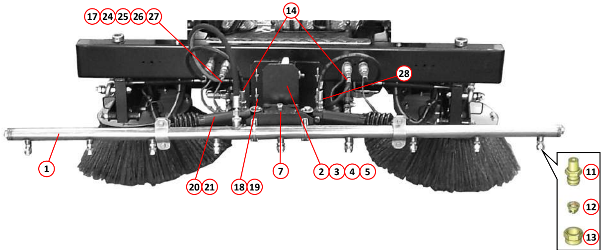
STREET WASH SPRAY BAR ARRANGEMENT
