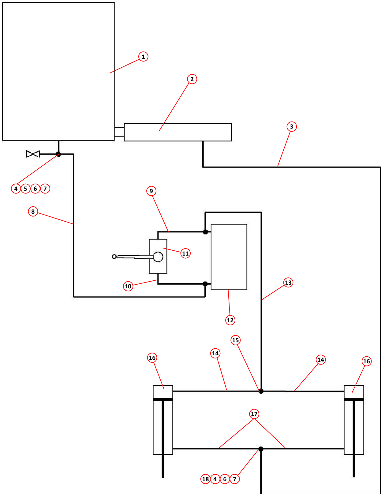
HYDRAULICALLY ASSISTED CAB-TILT CIRCUIT COMPONENTS
