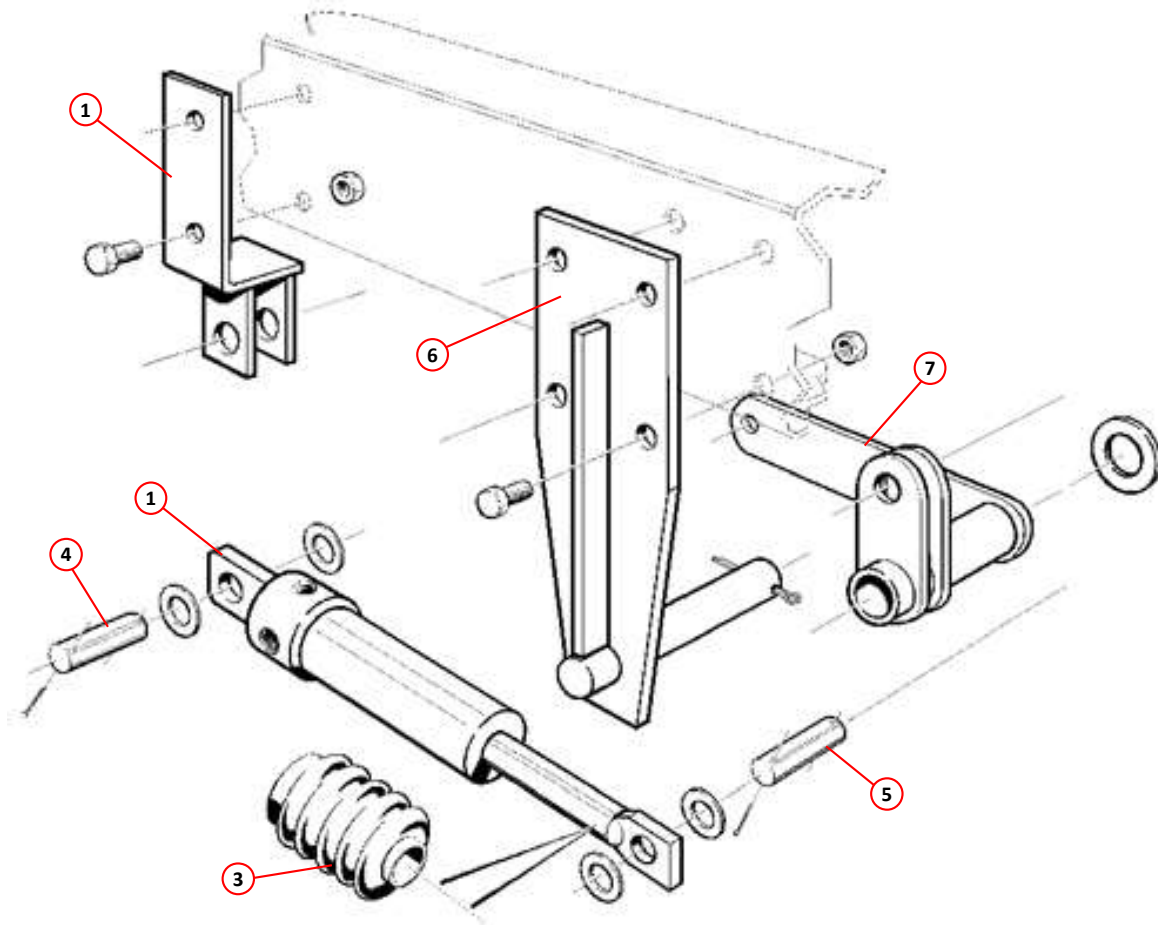
RH Sweep Assembly Illustrated, LH Assembly Similar
