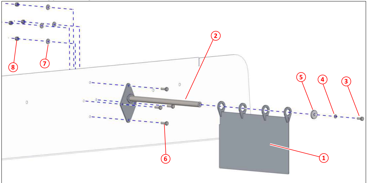
Figure 83: Deflector swing plate arrangement
