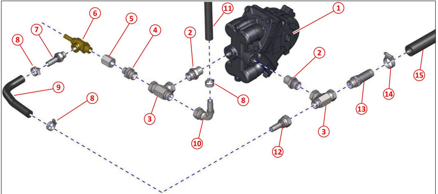
Figure 181: Water pump, twin diaphragm, low pressure, fittings
