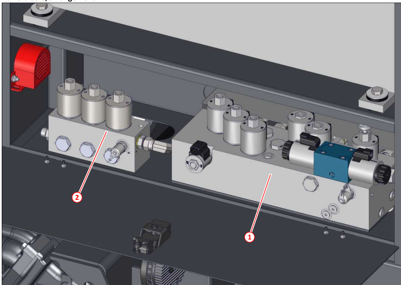
Figure 225: Valve blocks, arrangement
